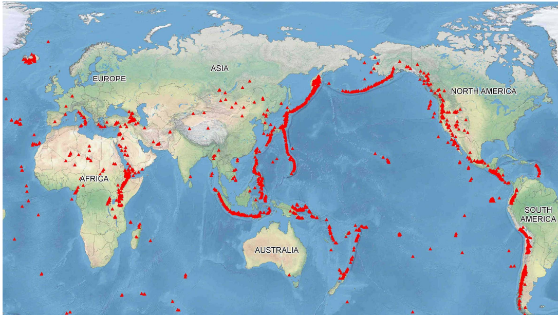
Distribution of volcanoes on Earth
