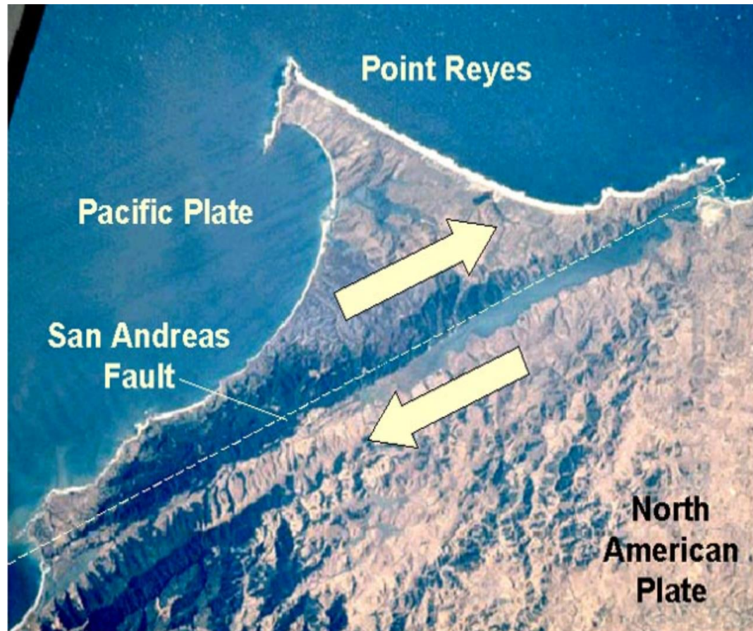
Satellite Image of San Andreas Fault
